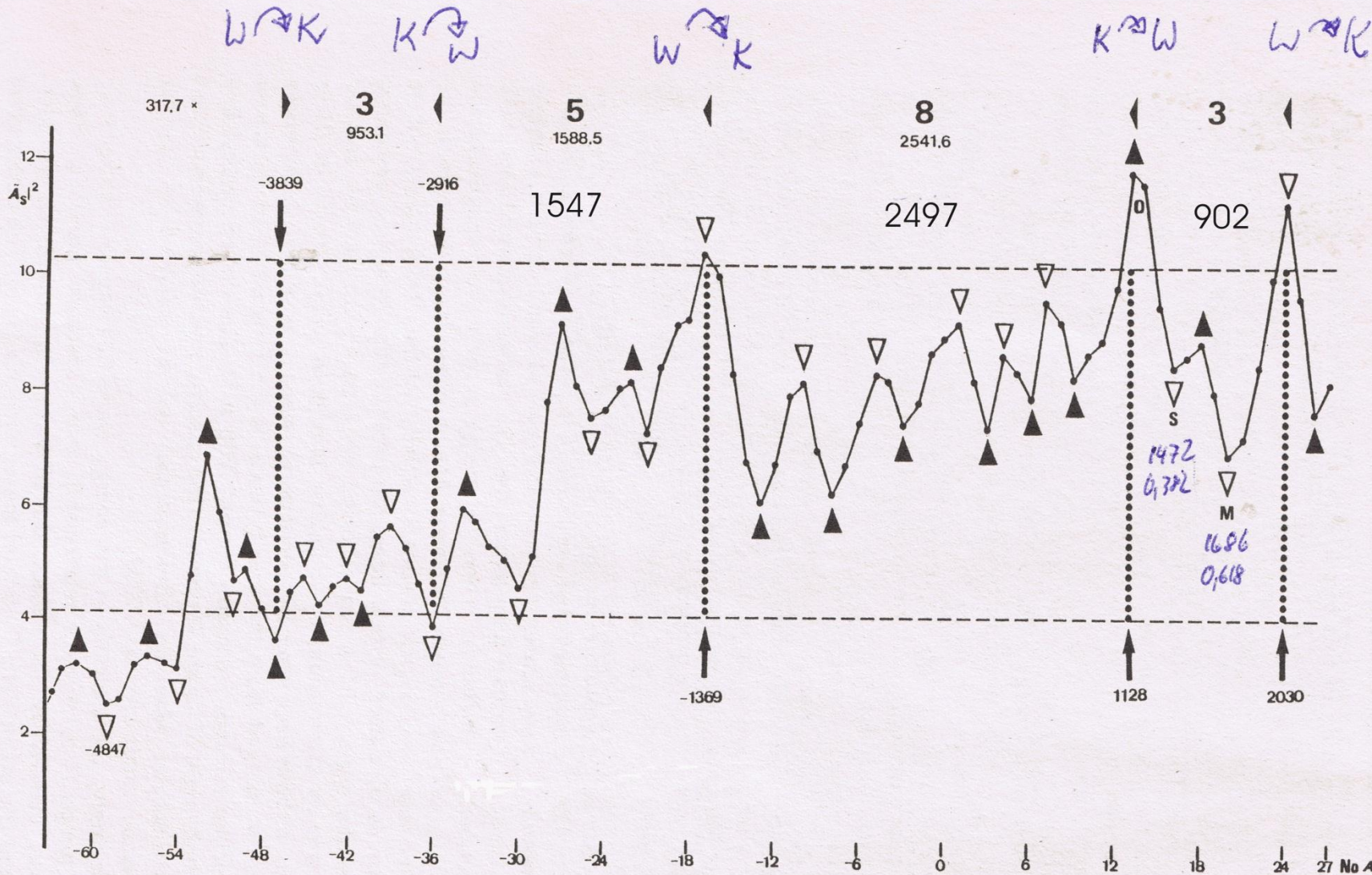
Figure 34: Combination of the consonant intervals major sixth (3 : 5) and minor sixth (5 : 8) emerging in solar system processes covering thousands of years. The intervals are indicated by vertical triangles and great numbers. The curve represents the supersecular variation of the energy in the secular torque wave, part of which was shown in Figure 19. The energy is proportional to squared values of the extrema in the secular torque wave ( A_s^2 ). Points in the curve represent epochs of extrema A_s numbers -64 to +28 (5259 B.C. to A.D 2347). The mean length of the cycle is 391 years. Black triangles point at maxima in the corresponding supersecular sunspot cycle; open triangles indicate minima. When the energy goes beyond quantitative thresholds, indicated by hatched horizontal lines, a phase jump occurs in the correlated supersecular sunspot cycle. These critical phases are marked by vertical dotted lines. A new phase jump is imminent about 2030. It points to a supersecular minimum, comparable with the Egyptian minimum (E) around 1369 B.C., a prolonged period of distinct cooling and glacier advance. The proportion 3 : 5 : 8, representing the major and minor sixth, just marks the intervals that separate those rare phase jumps set off by vertical dotted lines. The 317.7-year period of the triple conjunction of Jupiter, Saturn, and Uranus is, too, involved in this connection as indicated by small numbers beneath the great numbers at the top.
